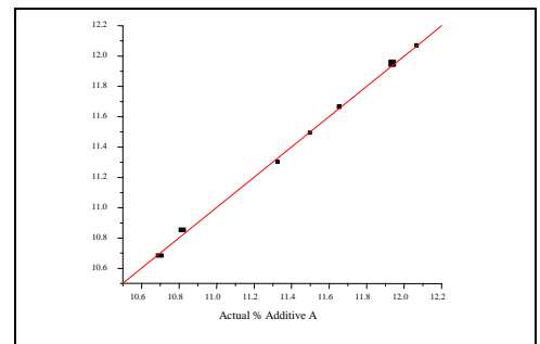
FIGURE 4: Actual additive dosage level versus the level predicted by the COAT® PortIA® System. Correlation is nearly 100%
